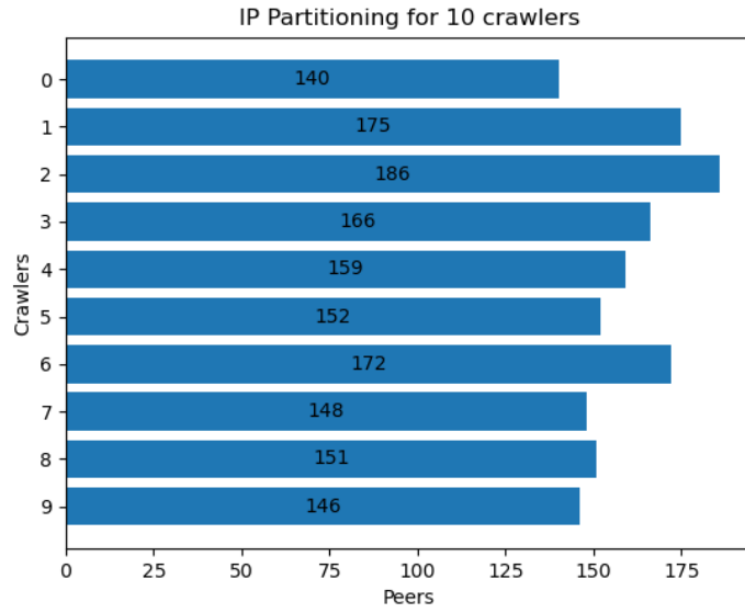
Figure 8: IP based partitioning for 10 crawlers
